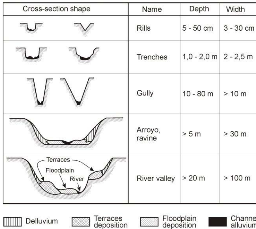
Figure 1. Water-erosional landforms in lowlands
