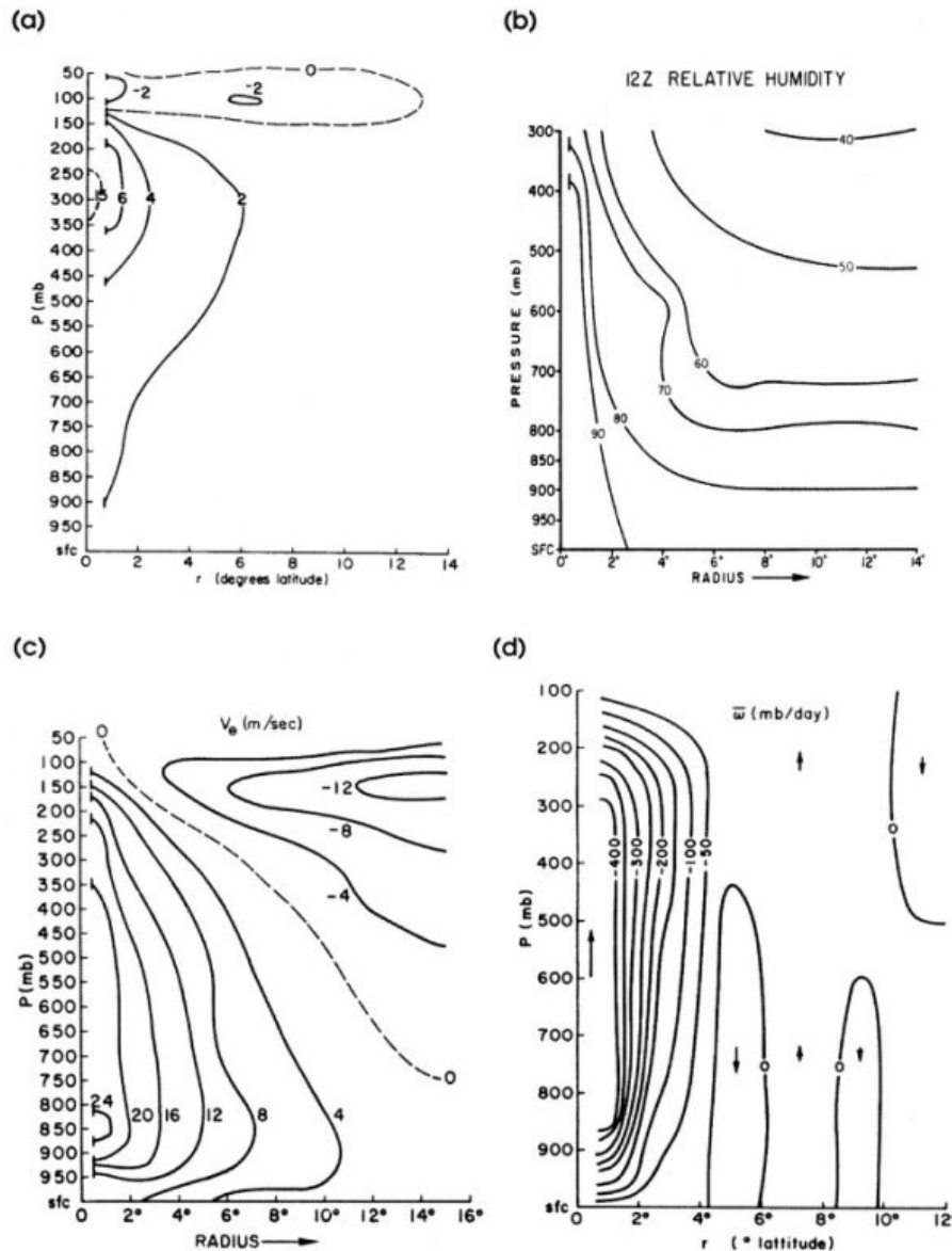
Figure 1. Two-dimensional cross section of an observed Typhoon (after Frank, 1977). (a) Temperature anomaly ( ^{\circ}\text{C} ), (b) relative humidity (%), (c) tangential wind ( \text{m s}^{-1} ), and (d) vertical velocity ( \text{hPa day}^{-1} ).
