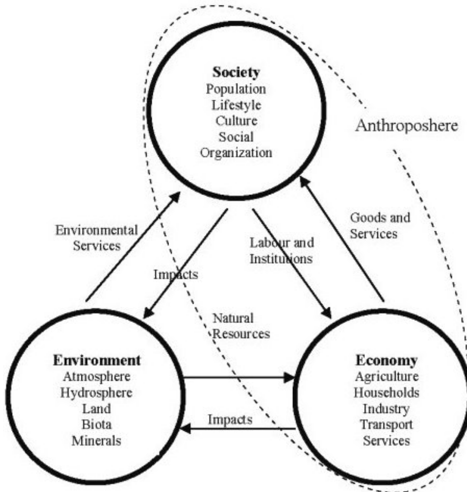
Figure 2. The three subsystems of the Earth system with their interactions
