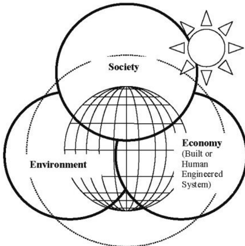
Figure 1: The grand scenario of the Earth system viewed as three interacting subsystems The Brundtland definition is from the point of view of human society. It is
