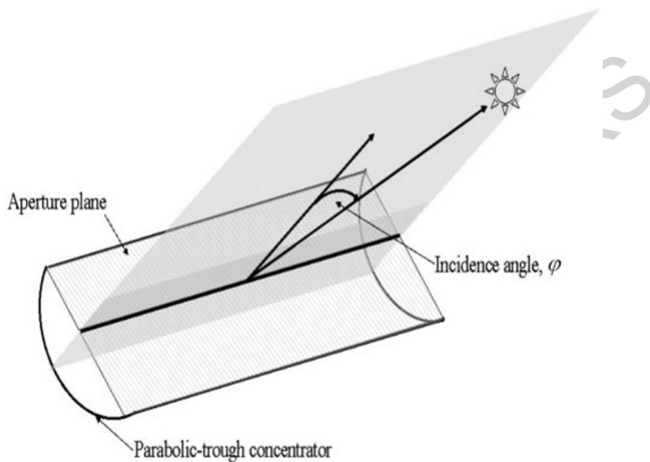
Figure 2: Correct positioning of a parabolic-trough concentrator
