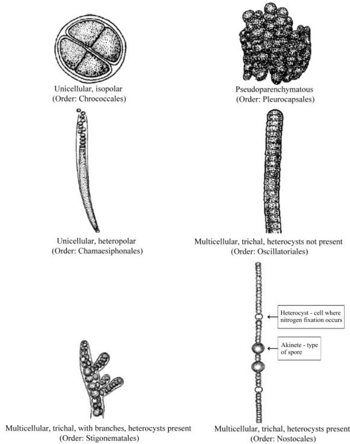
Figure 1 – Basic morphology of cyanobacteria
