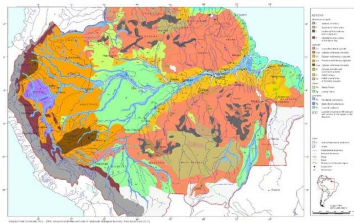
Figure 1. Situation map of the Amazon region, with main landforms, and location of Landsat image cut-outs.
